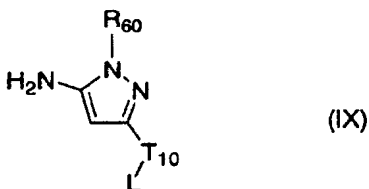
Formula (IX)
